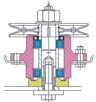
Bearings protected from string, wire, etc.
