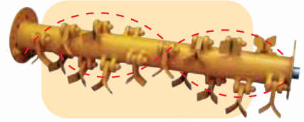
"OVERLAP" rotor with double row spiral flails
