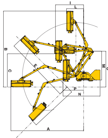
TJ 125 direct drive
